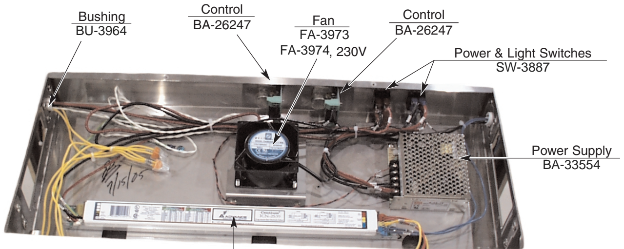
SC-36/2S with top panel removed
