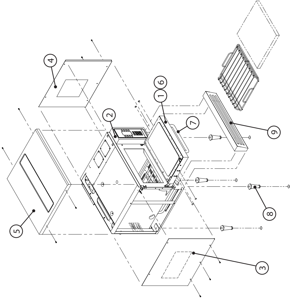
Starbucks Custom Oven (differences from original Tornado oven)
