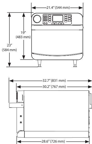
Figure 1: Encore and Encore 2 Oven Dimensions
