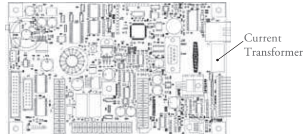
Figure 18: CT Location on Control Board
