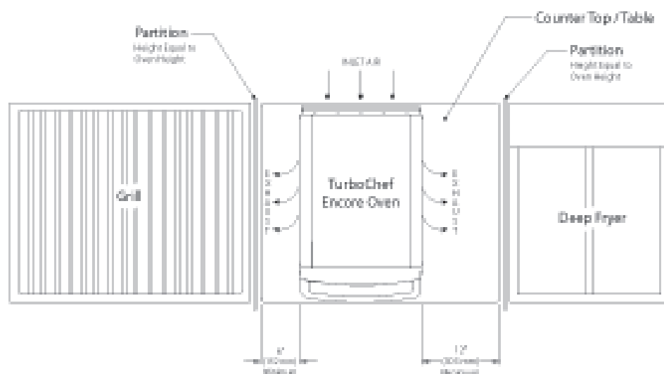
Figure 2: Installation Near Open Heat Source
