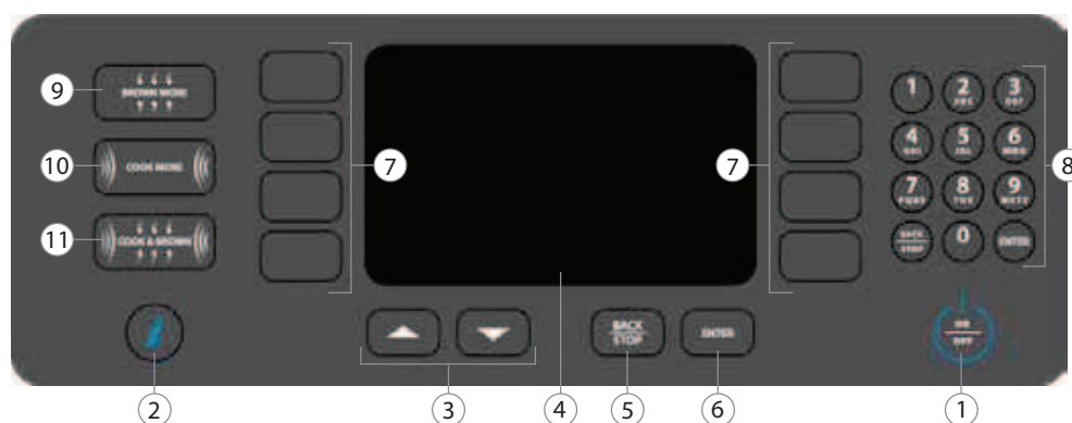
Figure 4: Oven Controls
