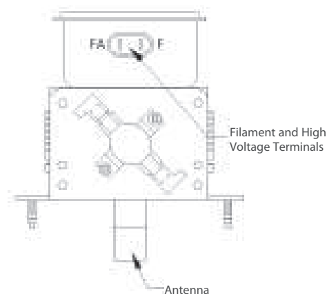
Figure 41: Magnetron Detail
