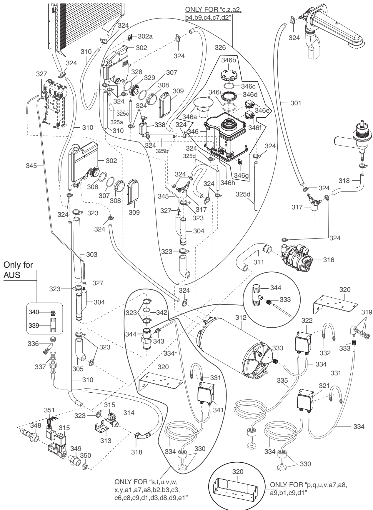
III. 595668W00_p5 Circuito idraulico/ Hydraulic circuit
